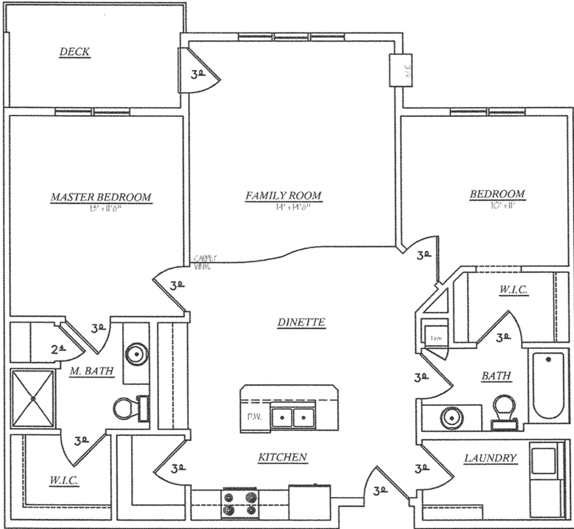
2-BEDROOM - UNIT C SCALE: 1/8" = 1'-0" 1130 SQ.FT
